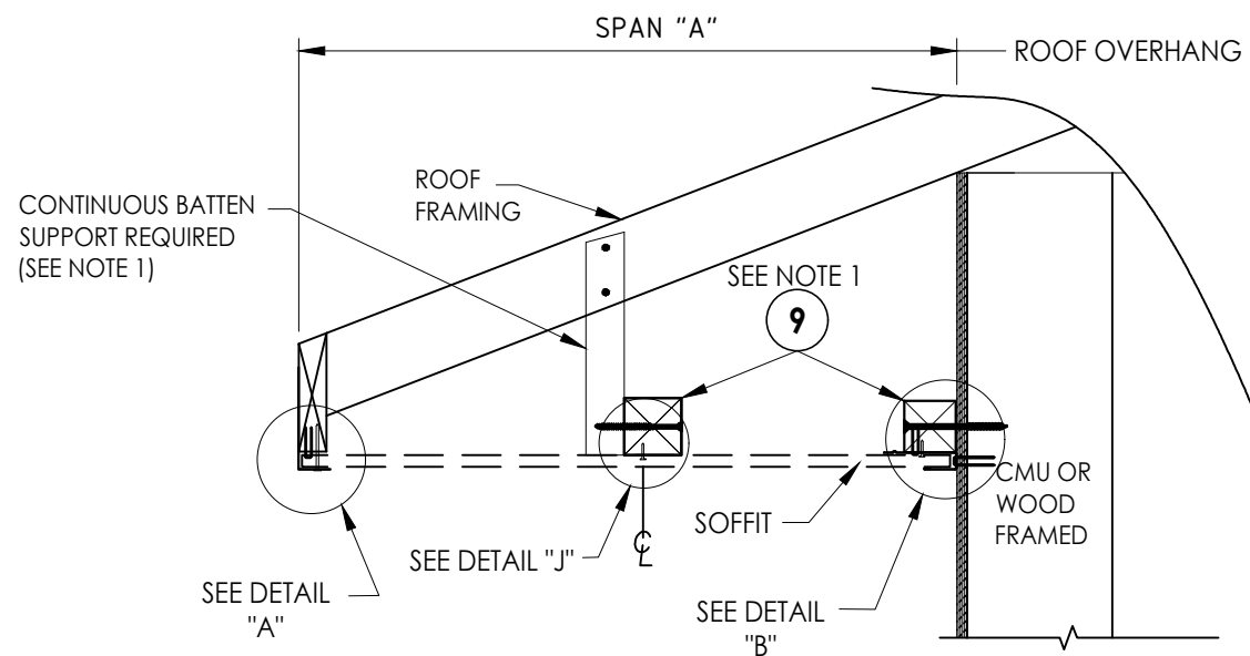
SIDE VIEW - DOUBLE SPAN w/ BATTEN
