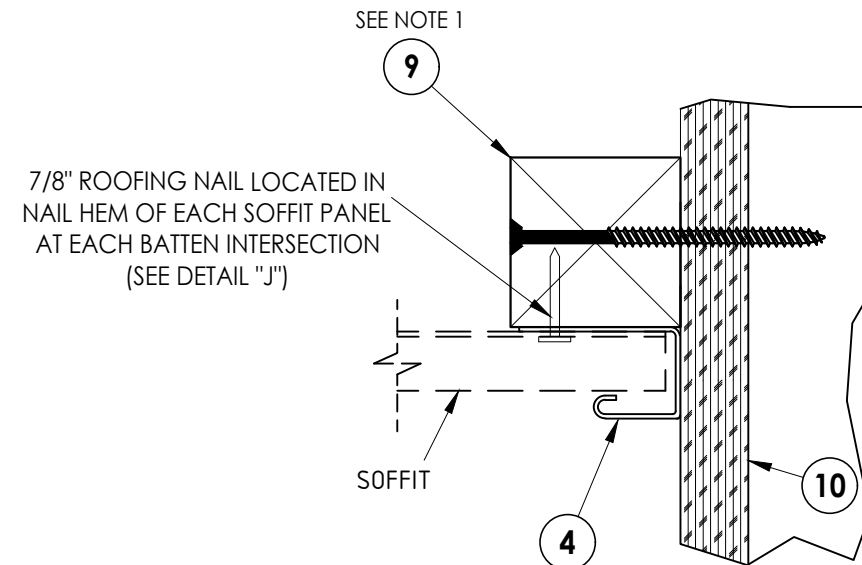
DETAIL "B"
