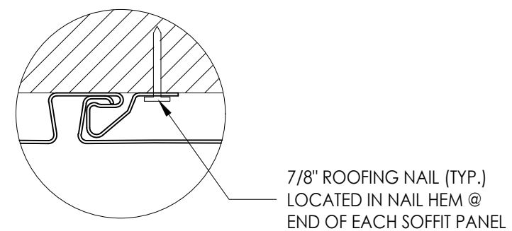
DETAIL "J"
