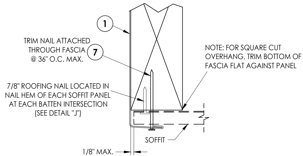
DETAIL "A"
