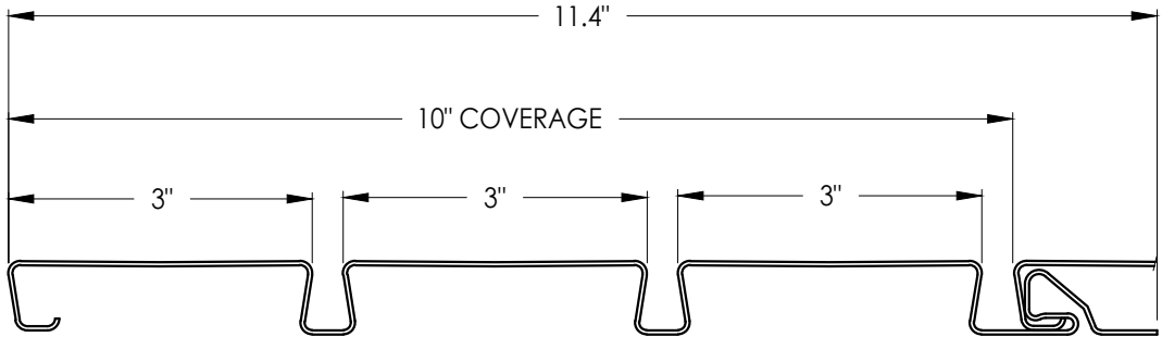
6 CHARTER OAK PANEL
