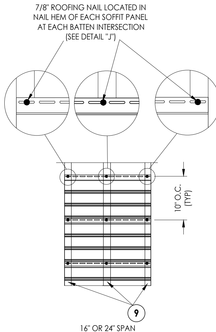
SIDE VIEW - DOUBLE SPAN w/ BATTEN
